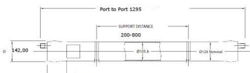
Frame, Front COMFORT+COMPACT Below: Pressure Vessel NF1000
