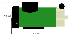
FWF System Boost Pump (LP Pump)
