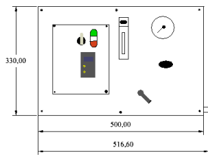
Frame, Front COMFORT+COMPACT Below: Pressure Vessel NF800
